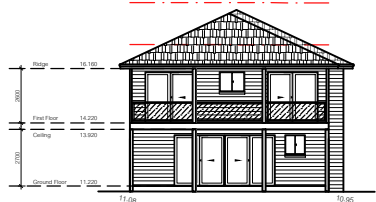
NORTH ELEVATION
