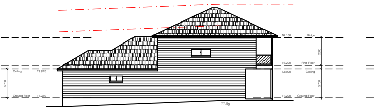
EAST ELEVATION
