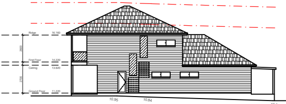
WEST ELEVATION
